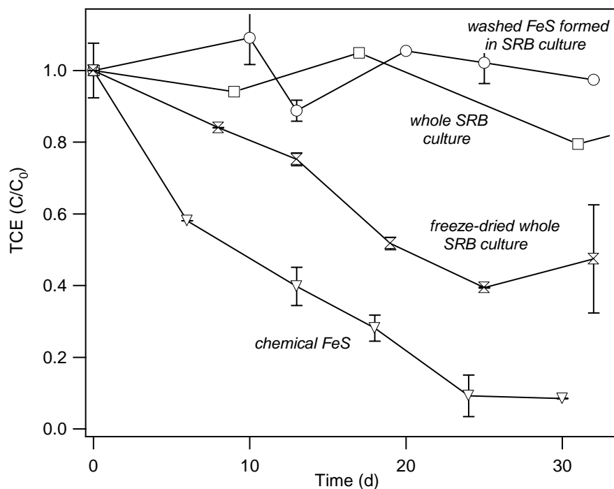
Figure 13. Disappearance of TCE over time in the presence of various iron sulfides precipitated in the absence and presence of sulfate reducing bacteria (SRB). 1 g/L FeSO 4 was added to induce FeS precipitation in the SRB cultures. All reactors with the exception of whole SRB culture contain 25 mM TAPS buffer at pH 7.5. Mineral concentrations were 5 g/L freeze-dried FeS formed in the SRB culture, (10 g/L) freeze-dried chemical FeS, and unknown in the whole SRB culture and the washed FeS formed in SRB culture (TP).
