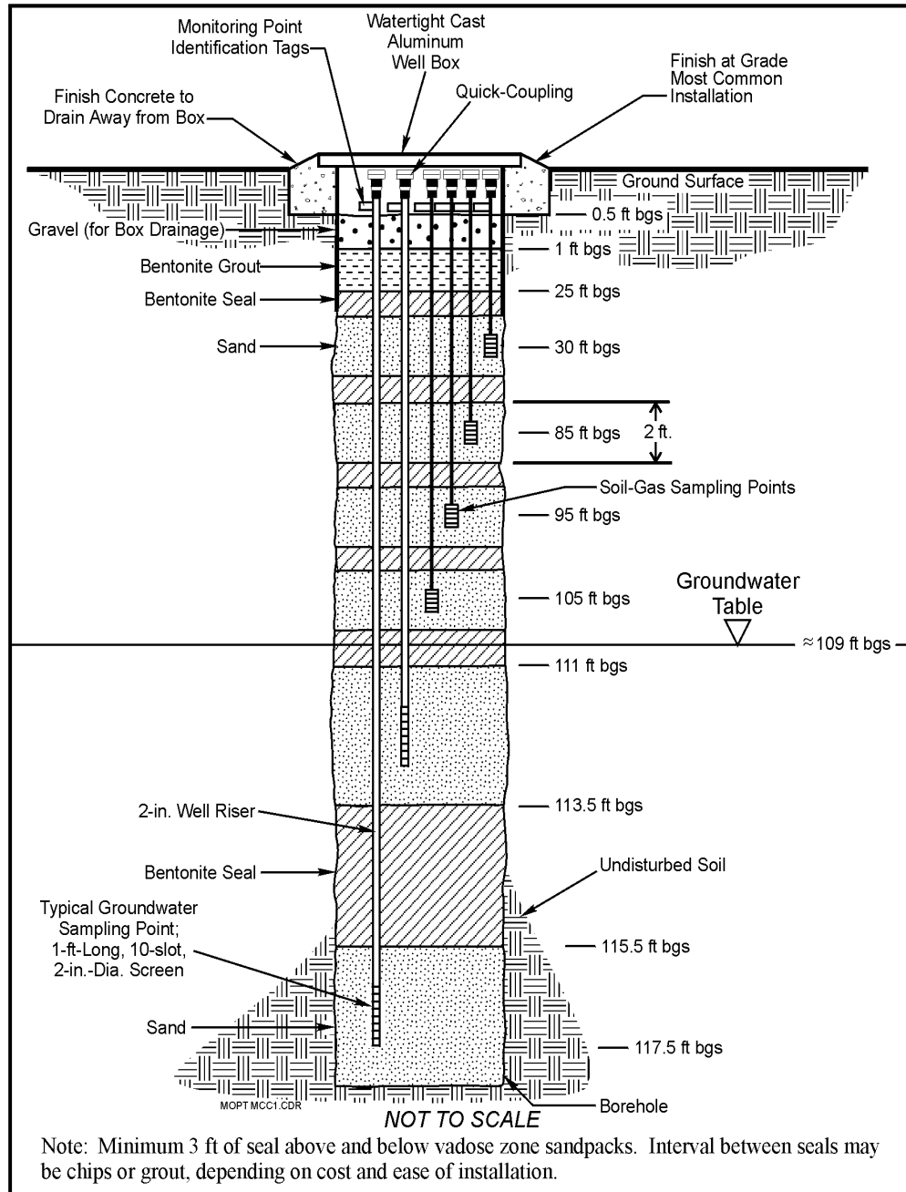
Figure 5. As-Built Layout for Multi-Level Soil Gas and Groundwater Monitoring Points.
